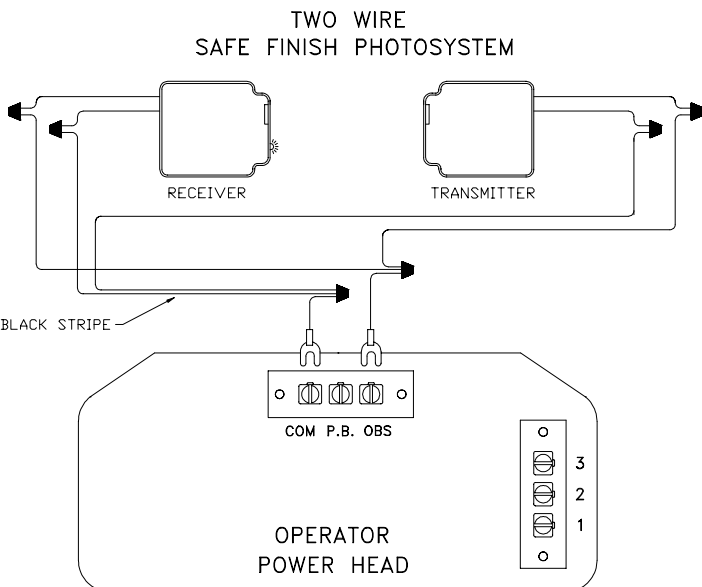
PHOTOCELL PARALLEL CONNECTION
