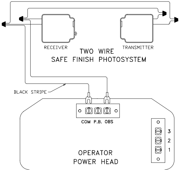
PHOTOCELL SERIES CONNECTION (RECEIVER FIRST)
