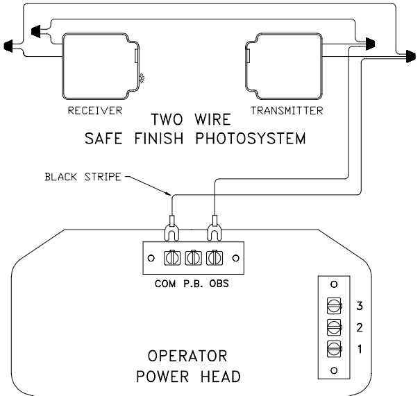
PHOTOCELL SERIES CONNECTION (TRANSMITTER FIRST)
